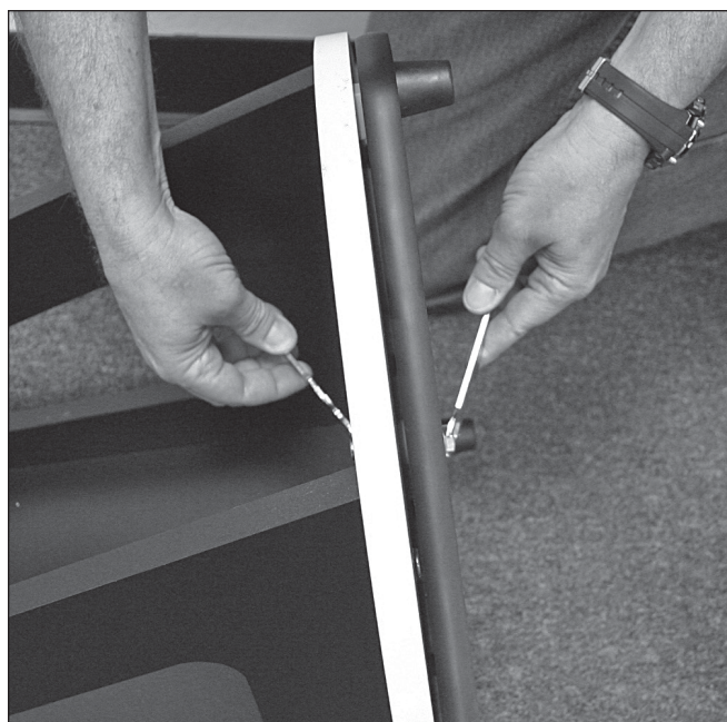
Figure 6. Use the two included open-end wrenches as shown to attach the bottom groundplate to the top groundplate.
