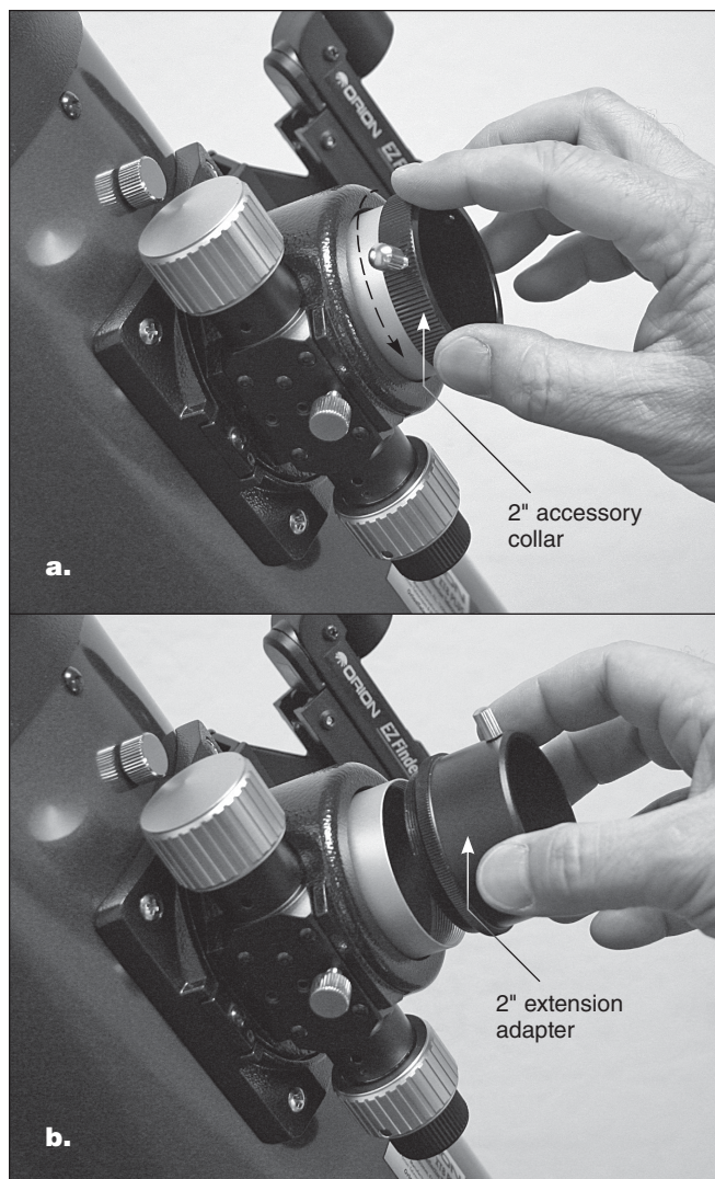
Figure 15. (a) Removing the 2" accessory collar (XT8 y XT 10 PLUS only), (b) Thread the 2" extension adapter into the focuser drawtube.
