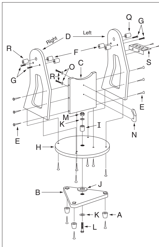
Figure 3. Exploded view of the XT PLUS Dobsonian base assembly.
