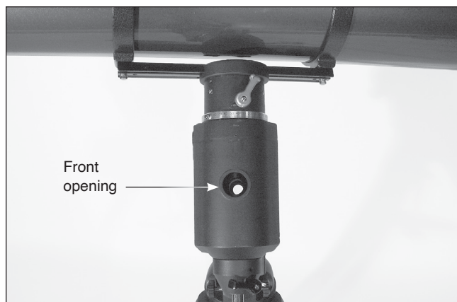
Figure 14. Rotate the declination axis until the hole in the declination shaft lines up with the front opening of the housing.
