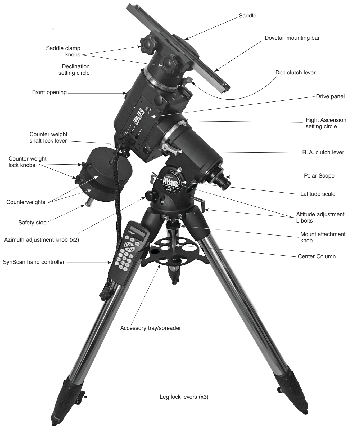
Figure 1. The Atlas EQ-G mount
