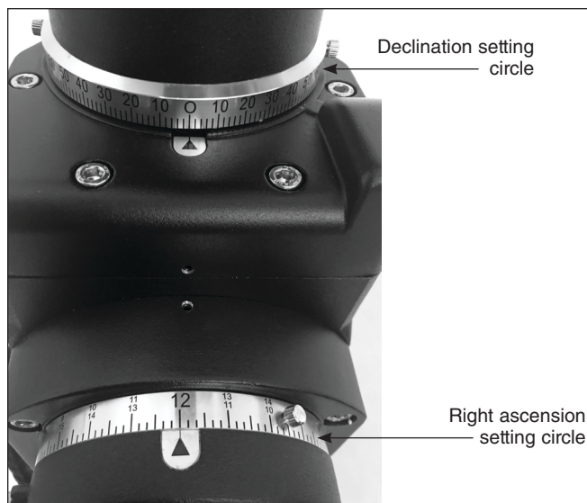
Figure 9. Use the right ascension and declination setting circles to find objects without the GoTo electronics, if desired
