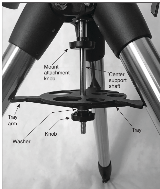
Figure 3. Install the accessory tray, flat side up, as shown. The three tray arms should press against the tripod legs.
