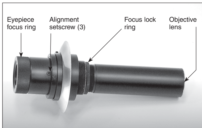
Figure 12. The polar axis finder scope
