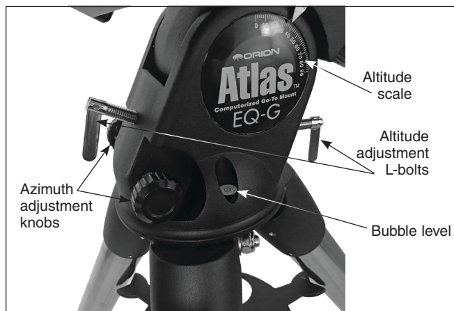
Figure 10. Use the altitude adjustment L-bolts and the azimuth adjustment knobs when polar aligning the mount.
