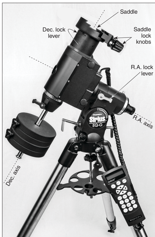
Figure 7. Before mounting a telescope, orient the saddle so the grooves run side to side, as shown here.
