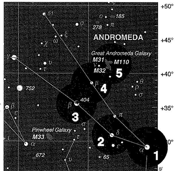
Figure 13. Starhopping is a good way to locate hard-to-find objects. Refer to a star chart to map a route to the object that uses bright stars as guideposts. Center the first star you've chosen in the finder scope and telescope eyepiece (1). Now move the scope carefully in the direction of the next bright star (2), until it is centered. Repeat (3 and 4). The last hop (5) should place the desired object in the eyepiece.
