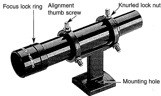
Figure 7: The 6x30 finder scope and bracket.
