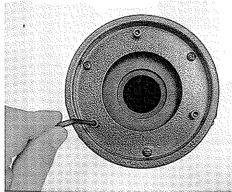
Figure 17: The three socket head cap screws that lock the primary mirror in place must first be loosened before any adjustments can be made.
