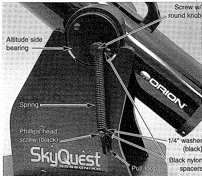
Figure 5. Close-up view of the CorrectTension System.
