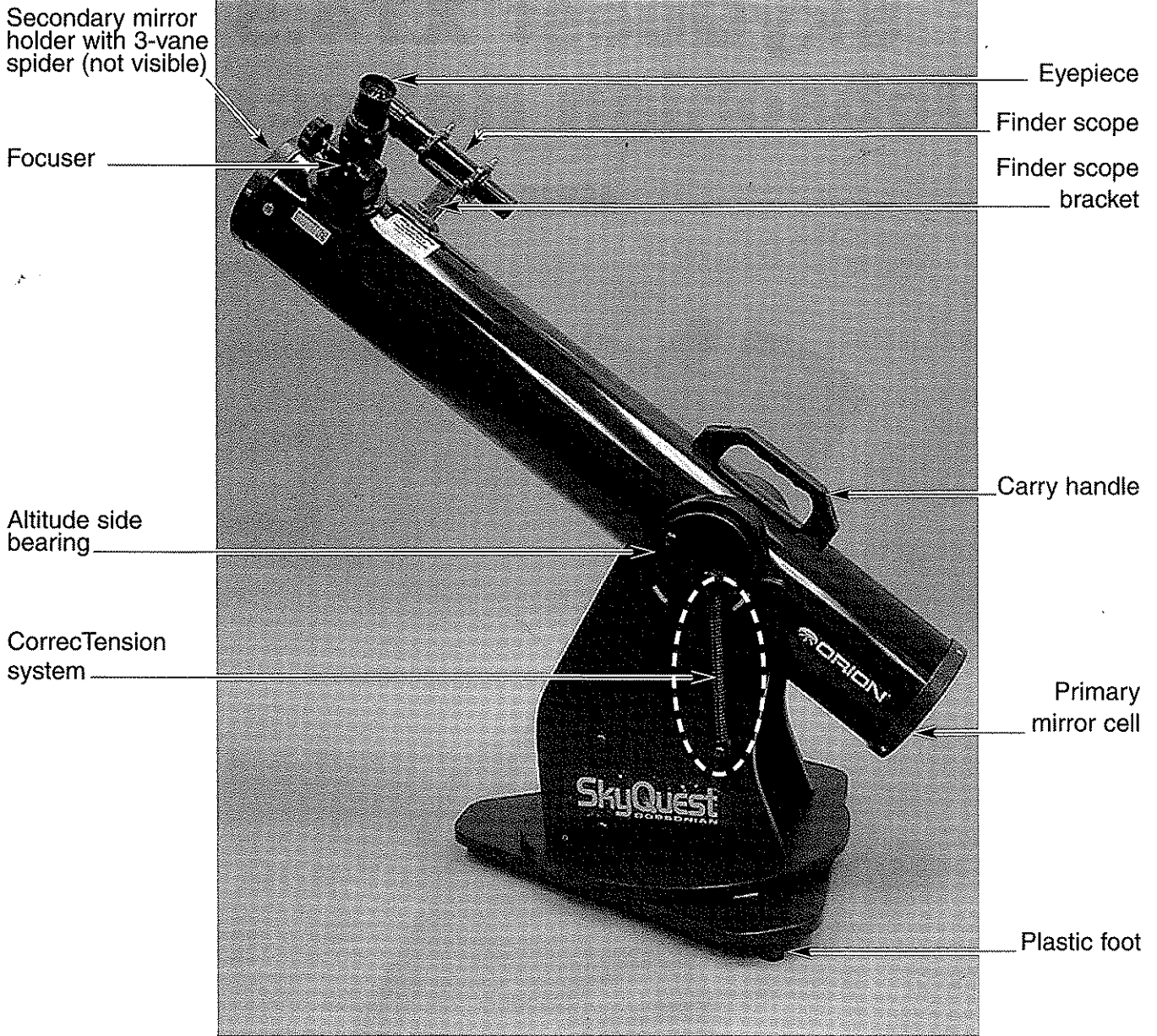
Figure 1. The SkyQuest XT4.5 parts diagram.
