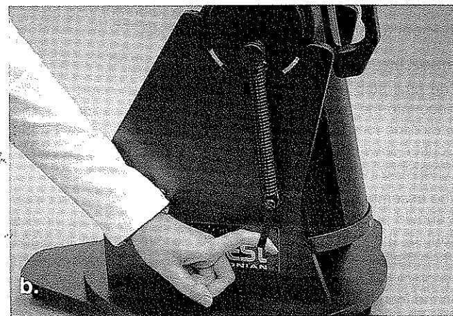
Figure 6: (a) To attach the spring to the base, grip the pull loop with your index finger and pull down on the spring. (b) While pulling down, slip the end ring of the spring over the screw head and onto the narrow part of the nylon spacer, then release the pull loop.
