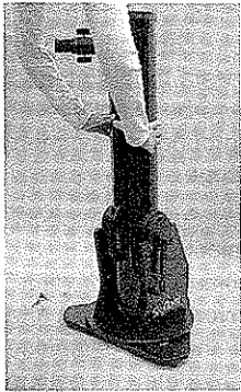
Figure 4. Set the optical tube on the "cradle" of the base so that the altitude side bearings on the tube rest on the white plastic "pads." Position the telescope as shown so that it won't fall down before the CorrectTension System is installed and engaged.
