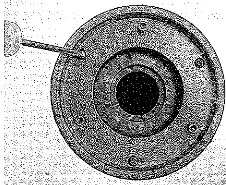
Figure 18: The tilt of the primary mirror is adjusted by turning one or more of the three Phillips head collimation screws.
