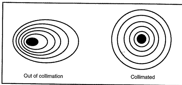
Figure 19. A star test will determine if a telescope's optics are properly collimated. An unfocused view of a bright star through the eyepiece should appear as illustrated on right if optics are perfectly collimated. If circle is unsymmetrical, as in illustration on left, scope needs collimation.
