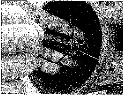
Figure 15: To center the secondary mirror under the focuser, hold the secondary mirror holder in place with your fingers while adjusting the center screw with the Allen wrench. Do not touch the mirror's surface!
