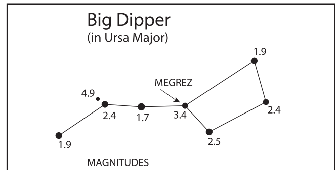
Figure 8. Megrez connects the Big Dipper's handle to its "pan". It is a good guide to how conditions are. If you cannot see Megrez (a 3.4 mag star) then conditions are poor.
