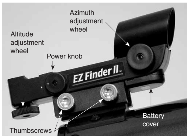
Figure 6. The EZ Finder II reflex sight
