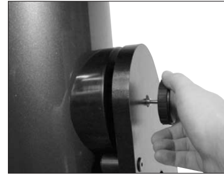
Figure 6. The retaining knob now goes through the shaft of the altitude encoder assembly before threading into the side bearing on the telescope tube.
