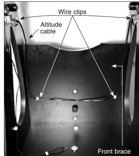
Figure 5a-b. Use the wire clips to secure the cables neatly to the base. (a.) For the XT6, XT8, and XT10 IntelliScopes, the altitude cable can be routed across the top baseplate. (b.) For the XT12 IntelliScope, the altitude cable is routed across the front brace.
