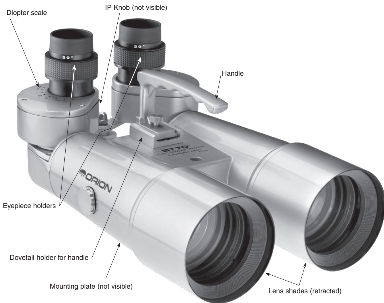
Figure 1. The Orion BT70 Binocular Telescope.
